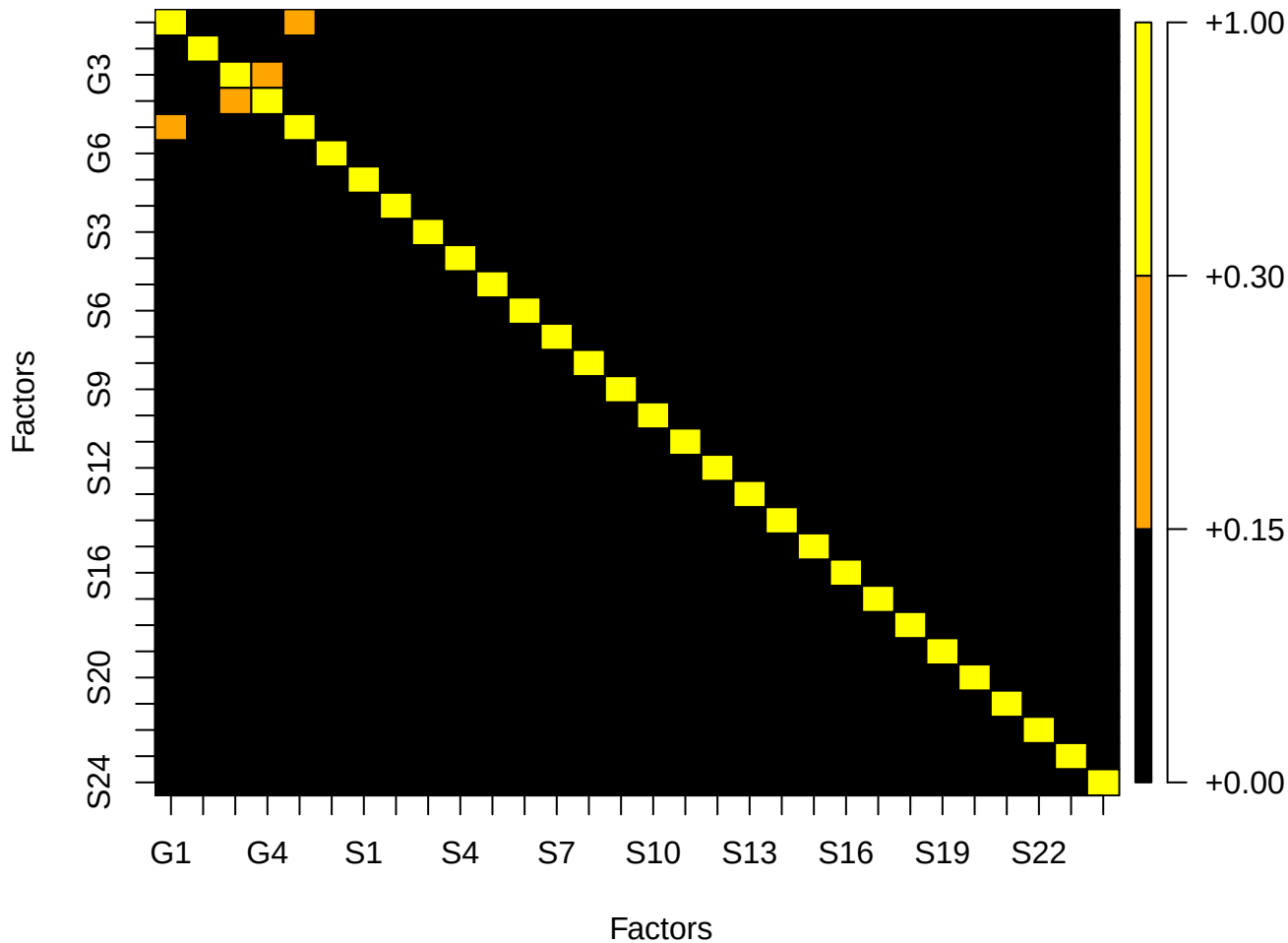
Absolute value of factor correlations (oblimin + target)
